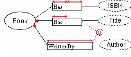
Fig. 10. 'Library' Ontological Commitment
